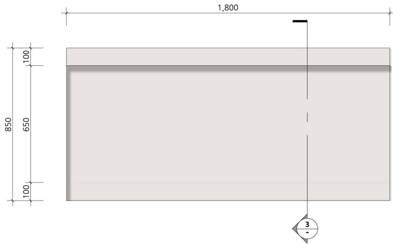
1 FRONT VIEW
