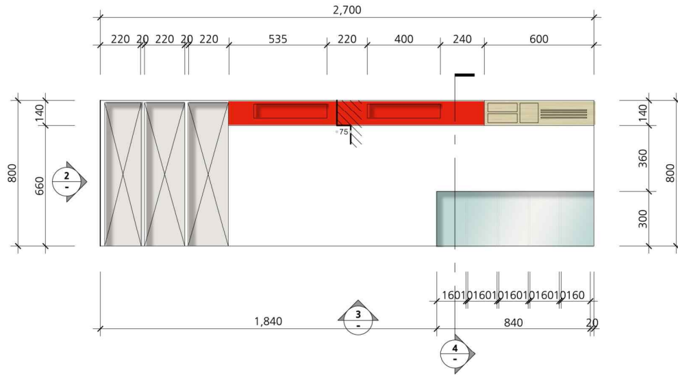
1 TOP VIEW
