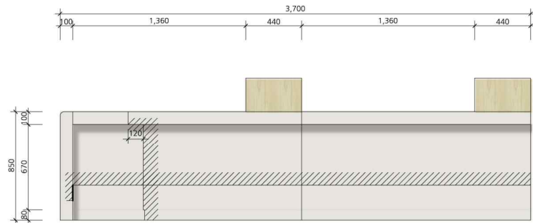
2 FRONT VIEW
