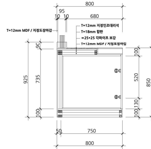
4 SIDE VIEW
