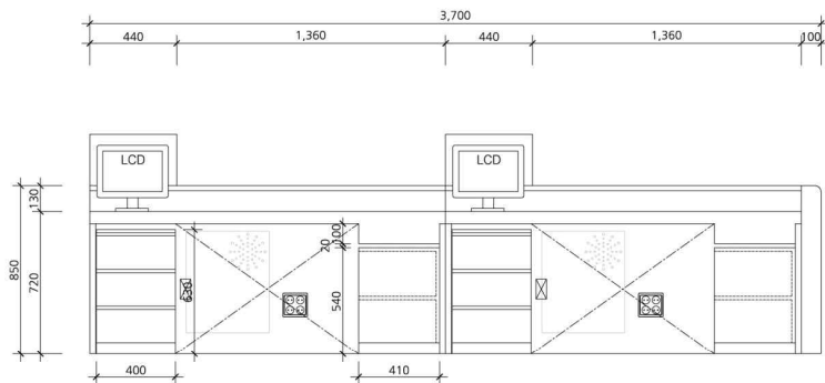
3 BACK VIEW
