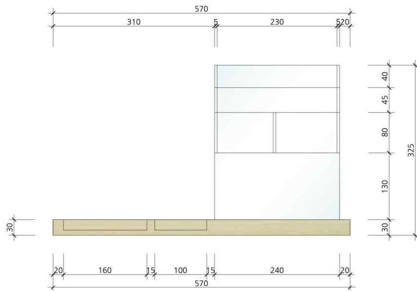
3 FRONT VIEW
