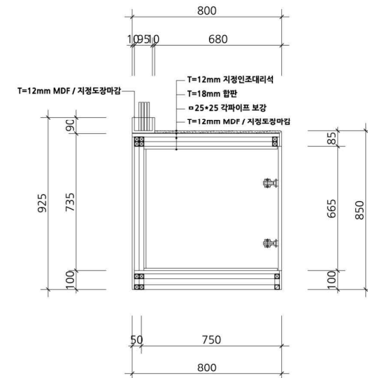
4 SECTION
