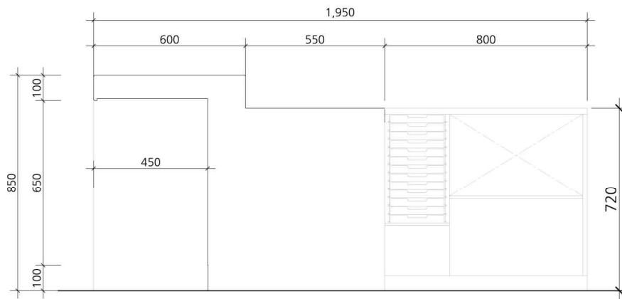
2 SIDE VIEW
