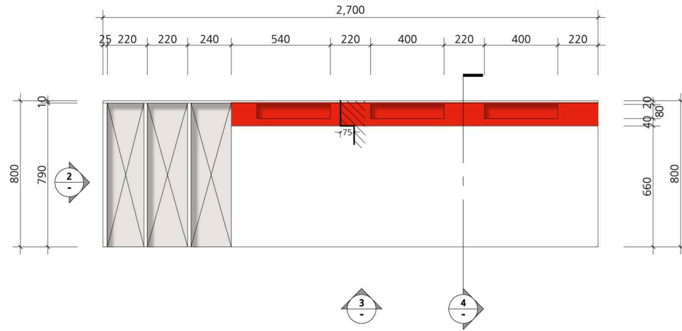
1 TOP VIEW
